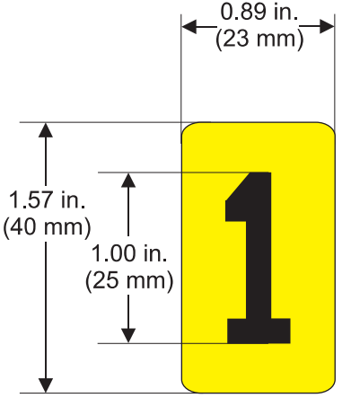
For horizontally oriented mounting Item 3DHKYxxx
